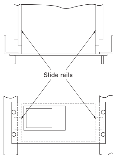
Mounting diagram
